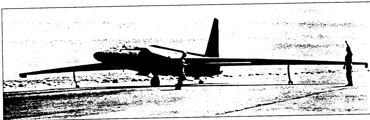
U-2 landing gear and pogos
