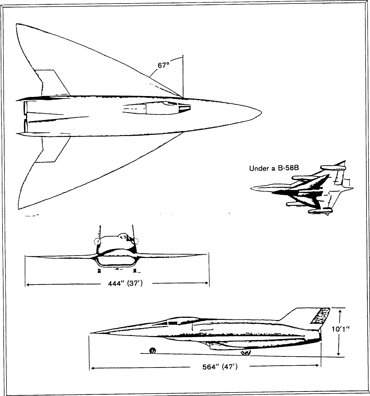
Convair FISH
