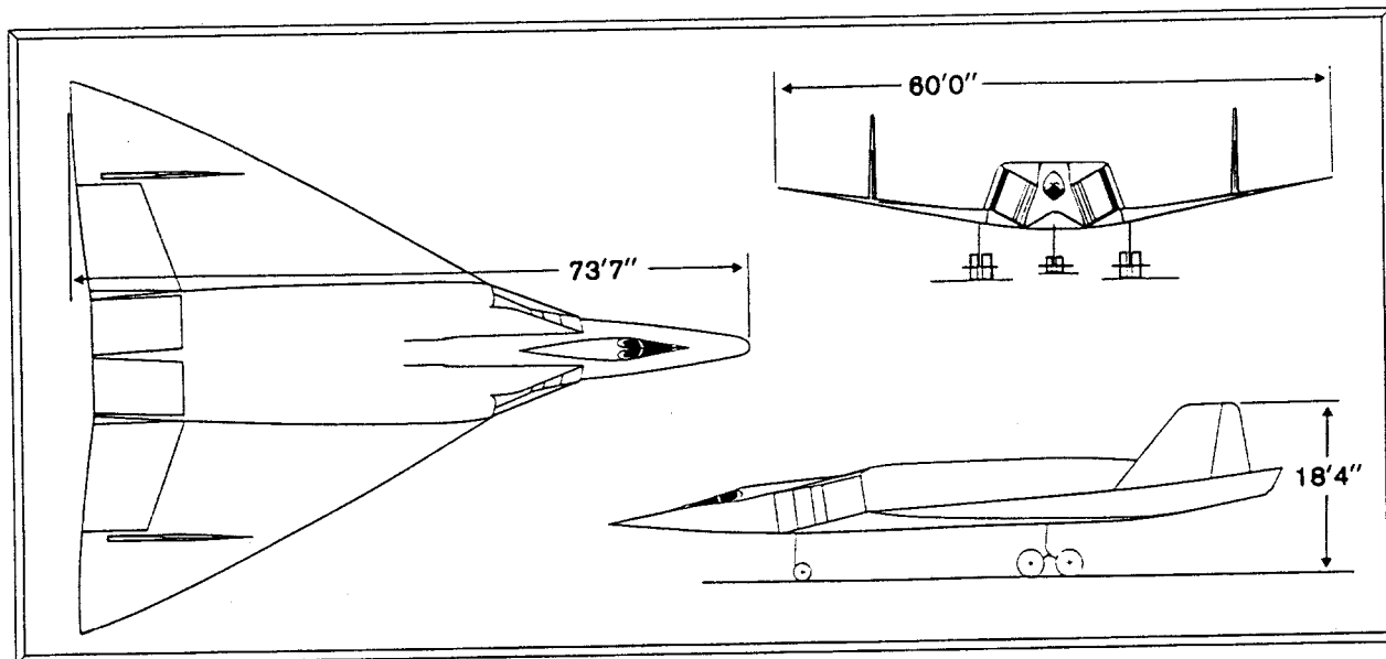
Convair KINGFISH
