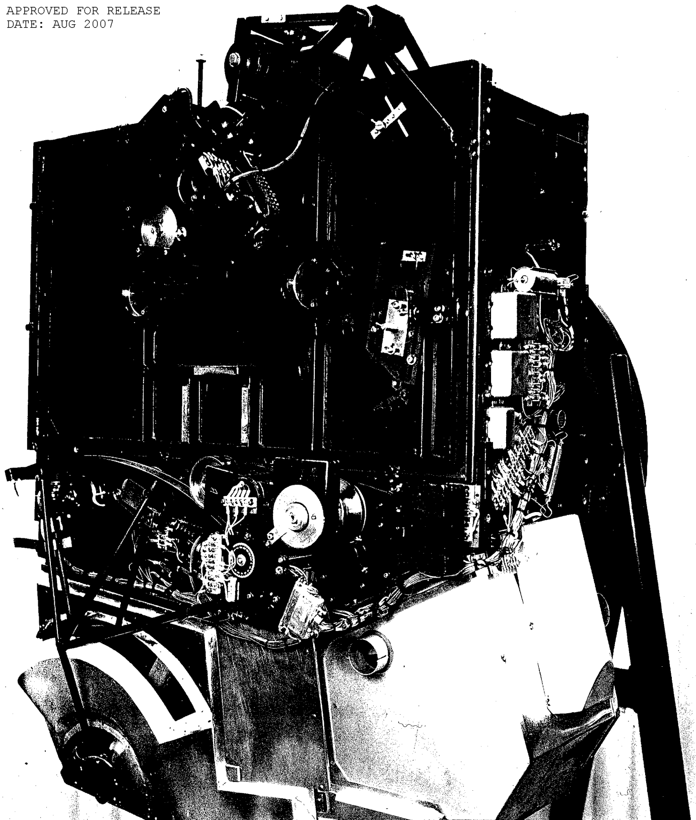
OXCART Eastman Kodak Type II Camera carries two 4200 feet rolls of film. It has a 21 inch focal length lens and with a design objective of 1 1/2 feet ground resolution from 85,000 - 90,000 feet.
